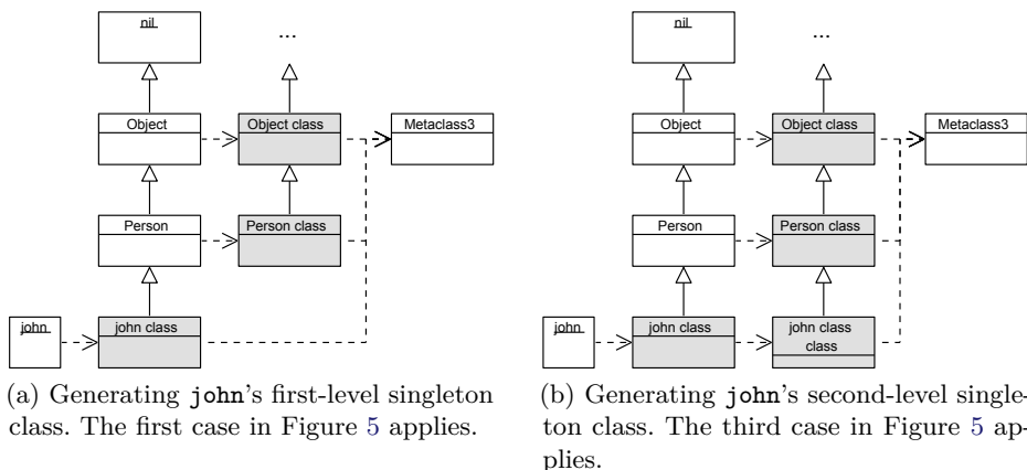
Figure 7. Generating john 's first-level and second-level singleton class. We do not need to generate more singleton classes recursively.
